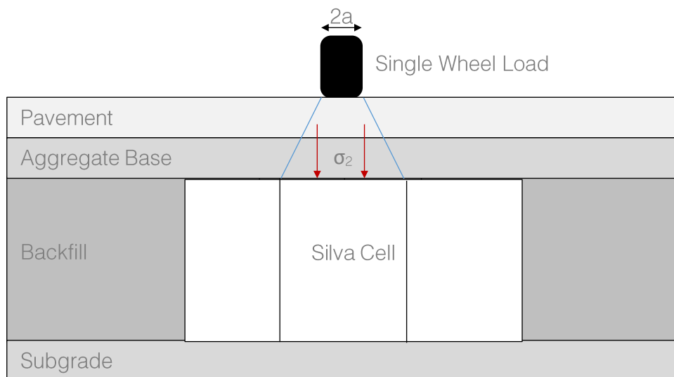
Figure 8: Configuration for Ultimate Load Calculation
